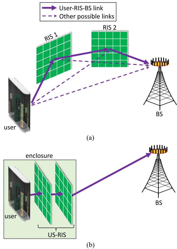
Fig. 6. Different systems employing multiple cooperative RISs. (a) Multiple cooperative BSS-RIS-aided communications. (b) Multi-layer US-RIS-aided communications.
